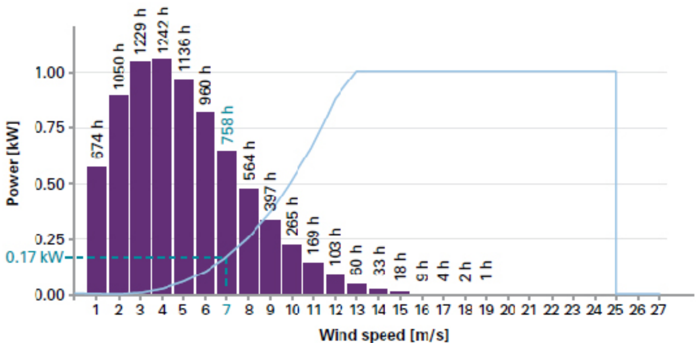
Figure 4, Calculation wind turbine production
